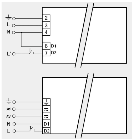
Pic 3. Wiring with 4 core flex
