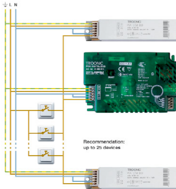
Pic. 6. SwitchDIM with several operation points
