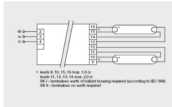
Pic 2. Wiring with two lamp configuration
