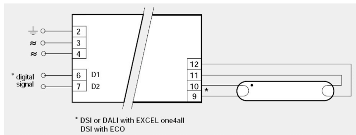
Pic. 7. DSI and Dali wiring diagram with 5 core flex
