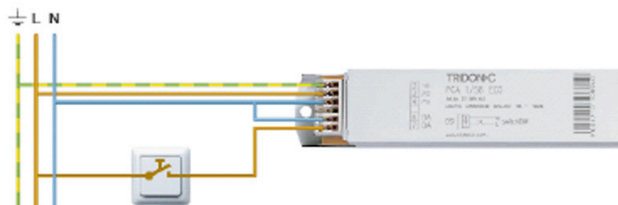
Pic 5. SwitchDIM with one operation point
