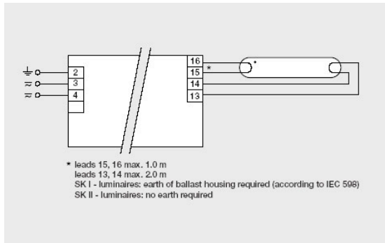
Pic 1. Wiring with one lamp configuration (Atco PC T5 Pro ballasts.)
